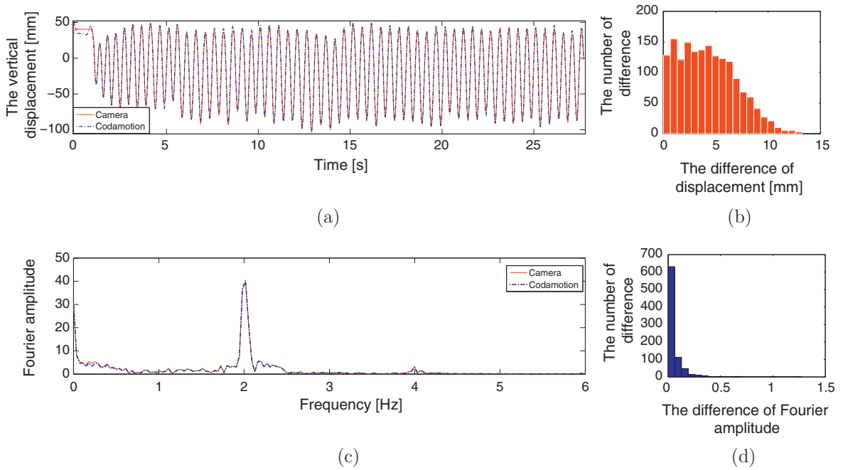
Fig. 6. (a) The comparison of two vertical displacements by subject 3 in Trail 3. (b) The histogram of the displacement difference values between the camera and Codamotion. The difference values are the direct distances of two corresponding points in two signals and not normalised. (c) The corresponding Fourier amplitude comparison with frequency from 0 to 6. (d) The histogram of the Fourier amplitude difference values between the camera and Codamotion.
