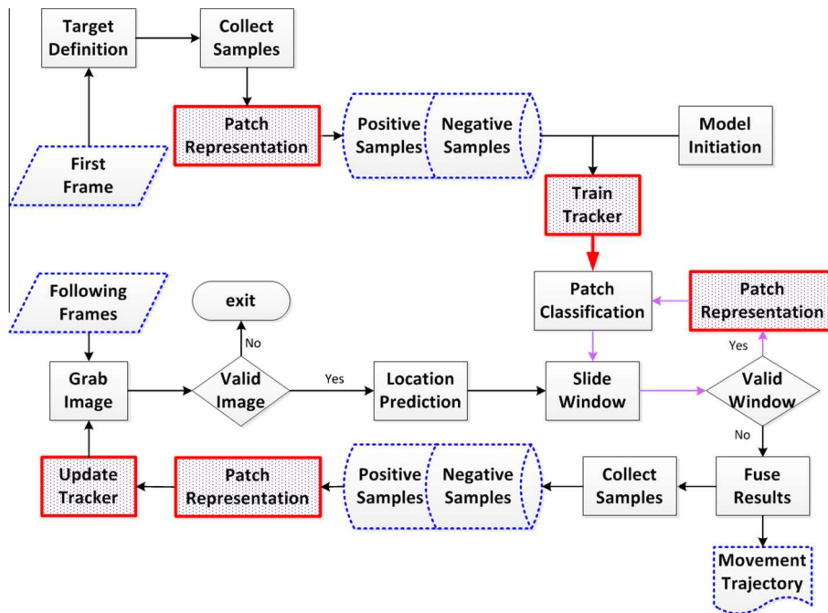
Fig. 1. The flowchart of our proposed system. Red boxes denote the main modules. (For interpretation of the references to colour in this figure legend, the reader is referred to the web version of this article.)
