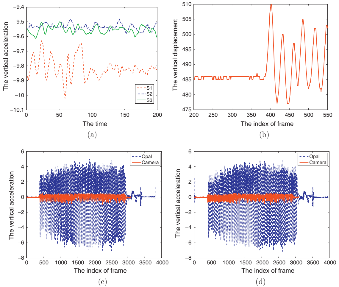
Fig. 5. (a) The acceleration examples of Opal sensors: subjects 1, 2 and 3 in Trail 1. (b) The displacement example of camera. (c) The two accelerations are aligned in time coordinate when the signal generated by Opal is downsampled to 57.7. (d) Same with (c) but the signal generated by Opal is downsampled to 60.
