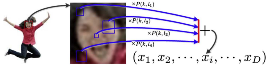
Fig. 2. The pipeline of image patch representation. The enlarged patch containing a face is used to explicitly illustrate the intrinsic mechanism but need not to be processed in our system.
