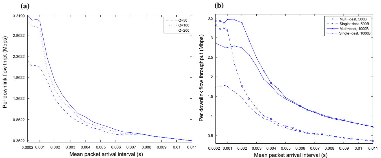
Fig. 9 Per downlink flow throughput versus mean Poisson packet arrival interval for a different queue sizes, b different packet sizes, 10 stations. a Flow packet size 500B. b Queue size 200 packets
