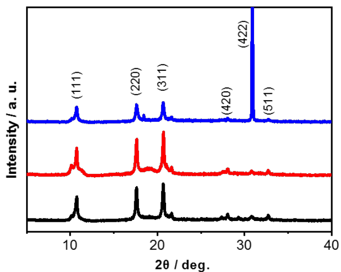
Figure S2. XRD patterns of FMPs prepared in NMP (black), pyridine (red) and aniline (blue).
