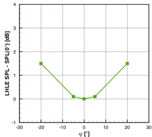
Figure 14. YawSens1 characteristic
