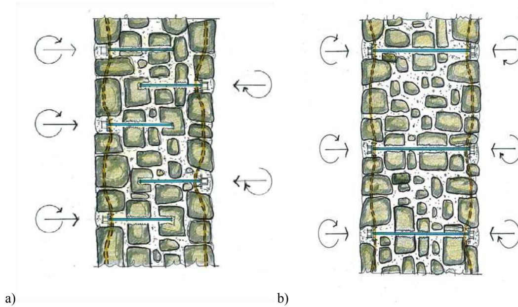
Figure 4: “Reticolatus” reinforcement work for poor quality masonry: vertical section.
