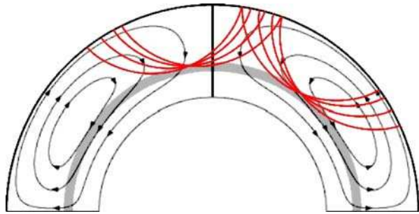
Fig. 3 Closed circulation lines: possible streamlines of meridional flow. Gray and red lines sound wave ( p mode) ray paths that can be used to measure the subsurface meridional flows using POLARIS high latitude
