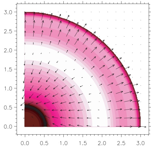
Figure 27. Velocity field on the (r, \phi) plane at z = 0.25 for Q = 32 , \sigma = 1 , \Omega = 0.1 and constant T bottom boundary, shown in Fig. 3. Arrows represent u_r and u_\phi and colour the sound speed perturbation \tilde{c}_s . \text{Max}(\tilde{c}_s) = 0.54 is the light shade between the two convection cells at r = 1.9 and \text{min}(\tilde{c}_s) = -0.03 the dark shade on the edge of the magnetic flux tube at r = 0.5 .
