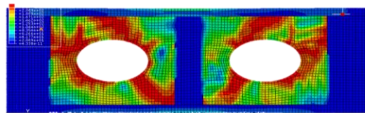
Figure 4: Shear failure mode of CFSS 200 x 75 x 15 x 1.5 LCB with 40x20 mm elliptical web openings
